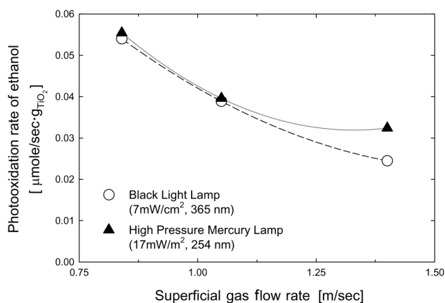
Fig. 5. Effect of gas velocity on the photooxidation rates of ethanol using the prepared \text{TiO}_2/\text{SiO}_2 photocatalysts ( \text{TiO}_2/\text{SiO}_2 800 g, T=30^\circ\text{C} , C_o=10,000 \text{ ppmv} ).
